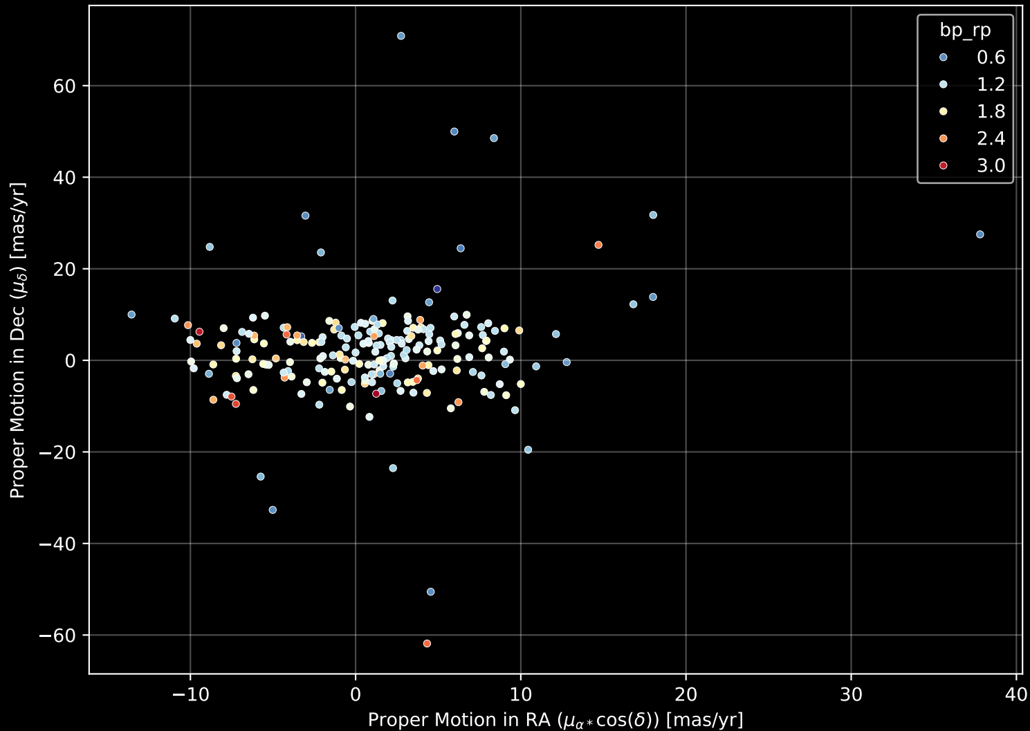
APOGEE DR17 Field: [264-33-C] Proper Motion Diagram (n= 224)
