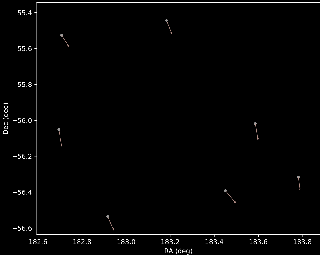
APOGEE DR17 Cluster 11 Proper Motion Vectors (n=7)
