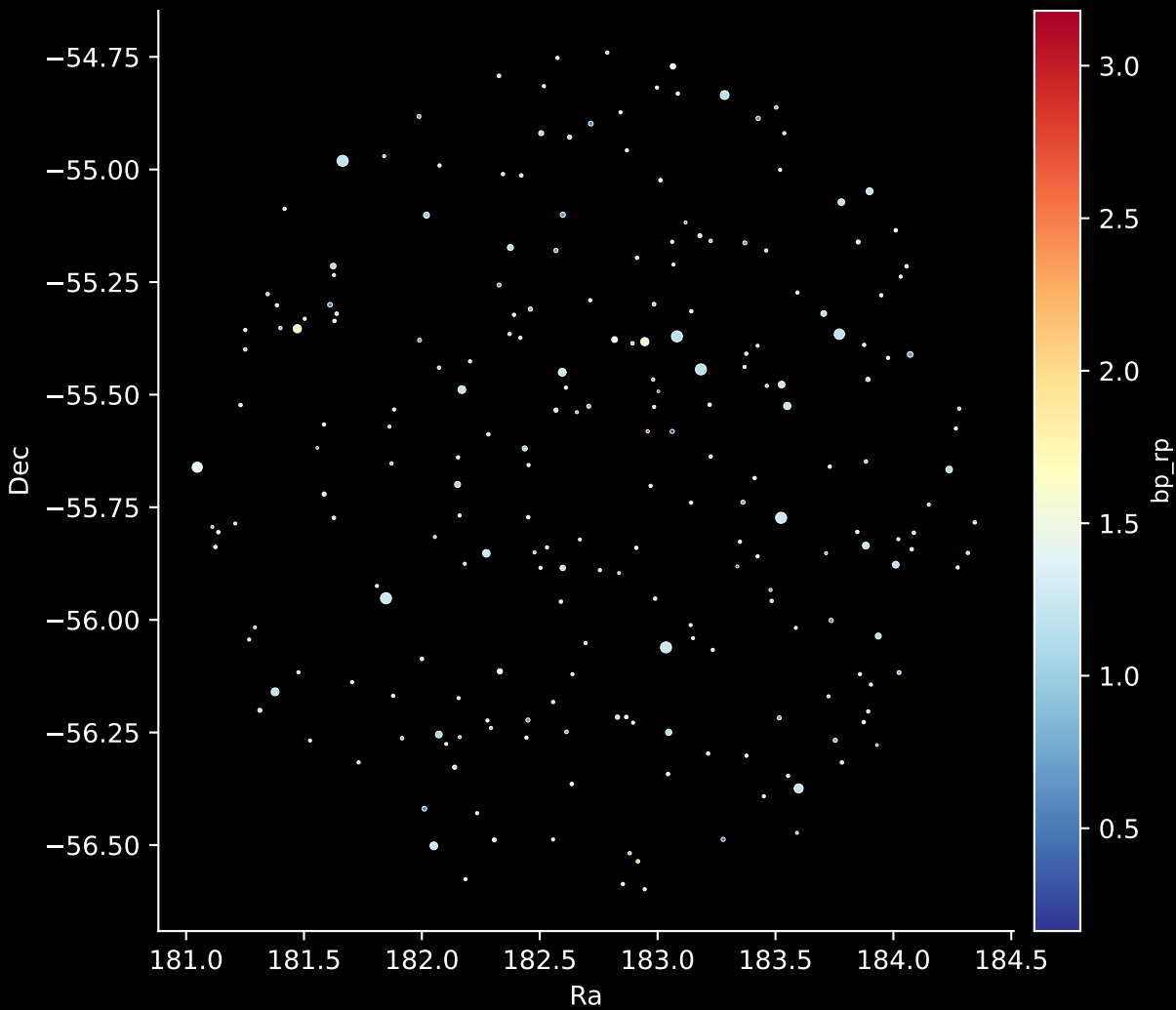
APOGEE DR17 Field: [264-33-C] Stars: 224
