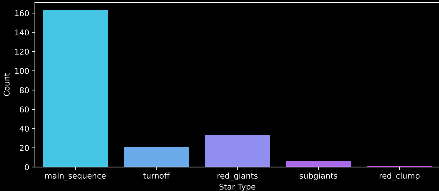
APOGEE DR17 Field: [264-33-C] Count plot of Star Type
