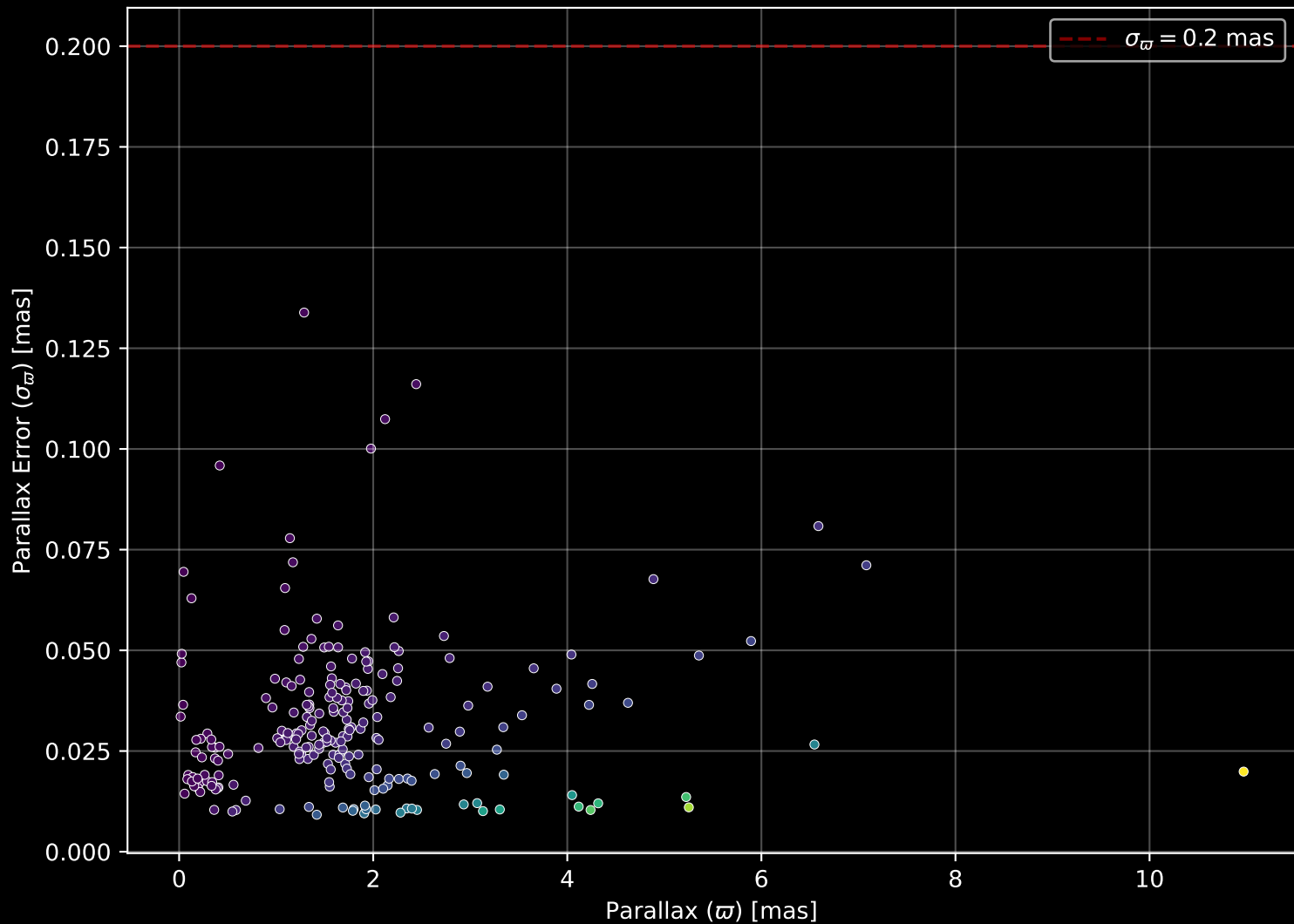
APOGEE DR17 Field: [264-33-C] Parallax Quality (n= 224)
