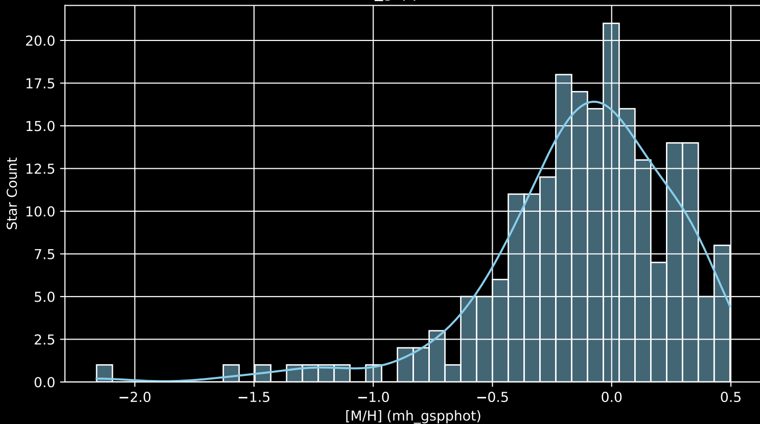
APOGEE DR17 Field: [264-33-C [M/H] (mh_gspphot) (n= 215)
