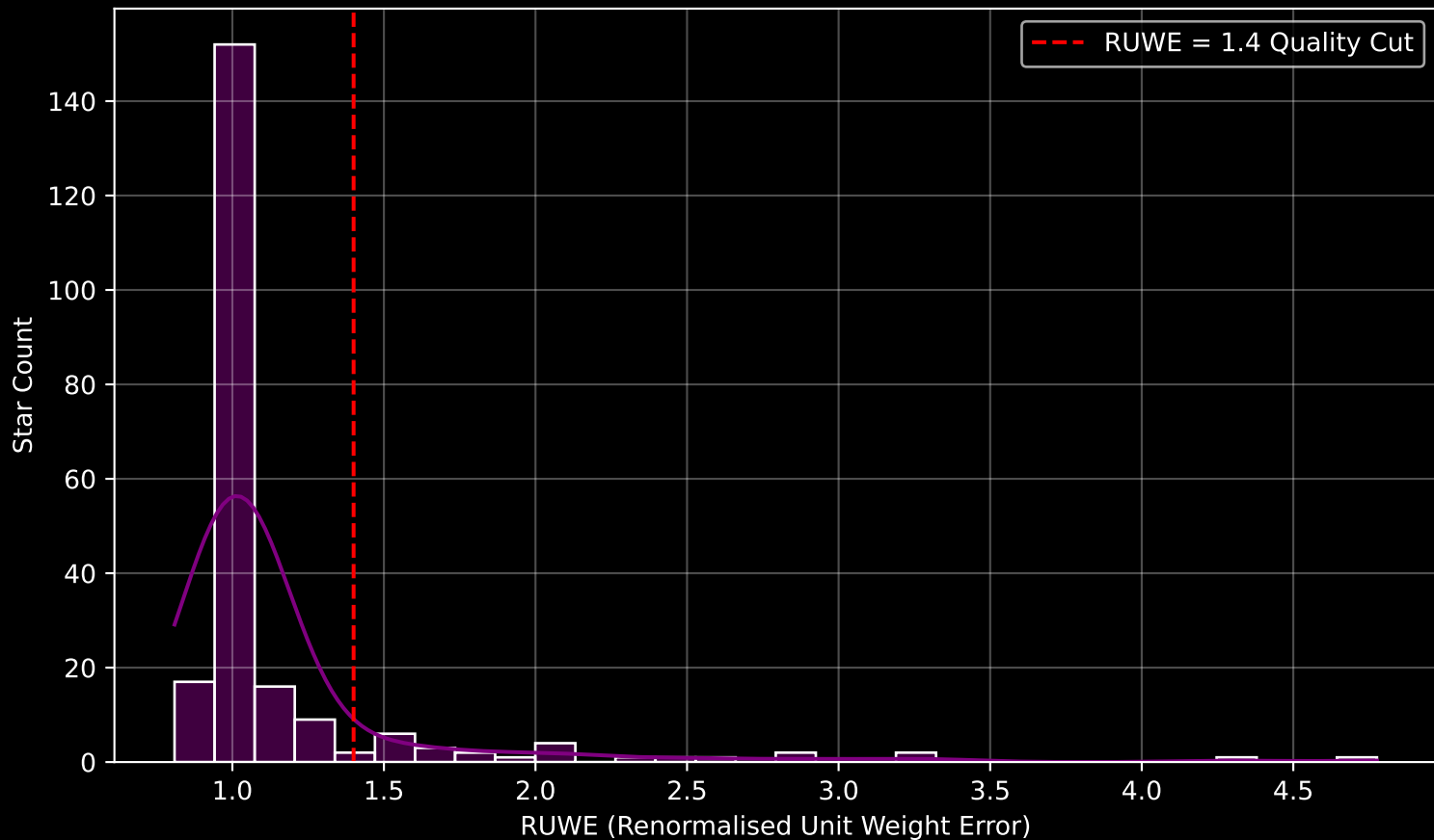
GAPOGEE DR17 Field [264-33-C] RUWE Distribution (n= 221)
